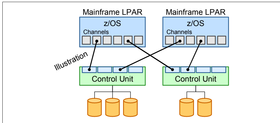
Figure 2-10 Basic shared DASD
