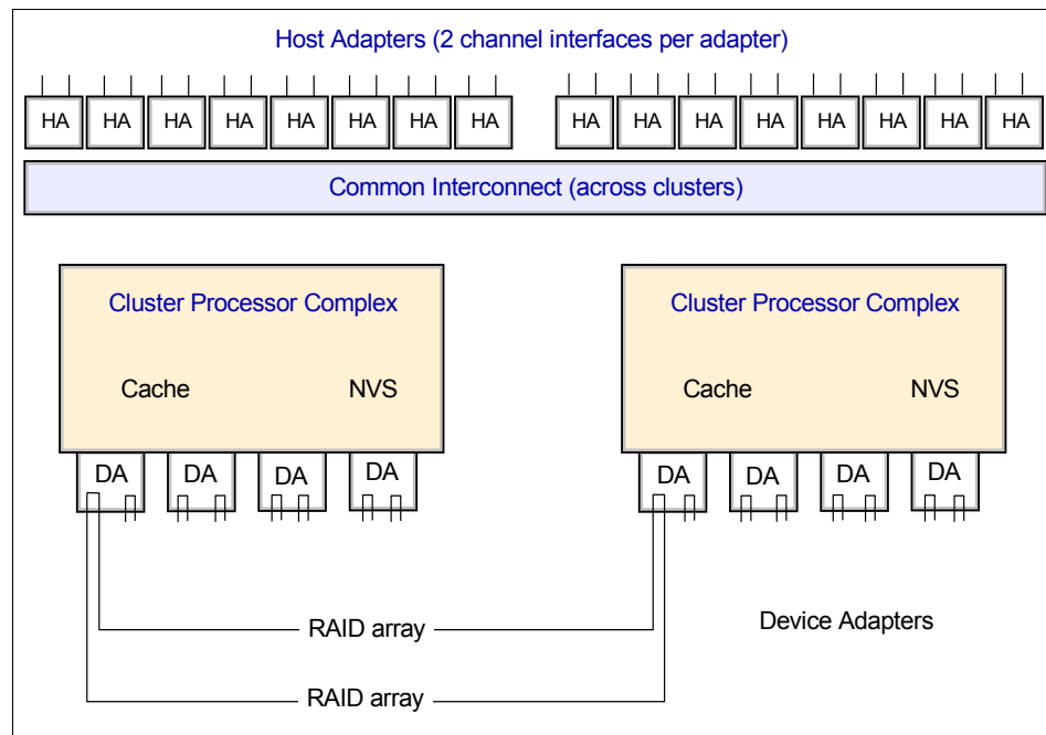
Figure 2-9 Current 3390 implementation
