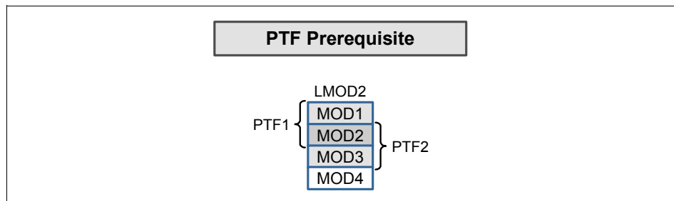
Figure 17-8 PTF prerequisite
