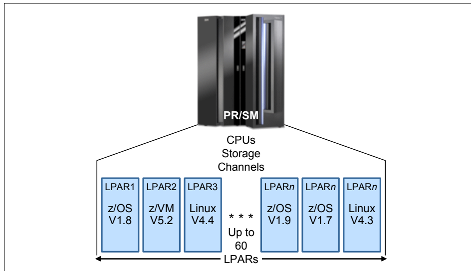
Figure 2-7 Logical partitions
