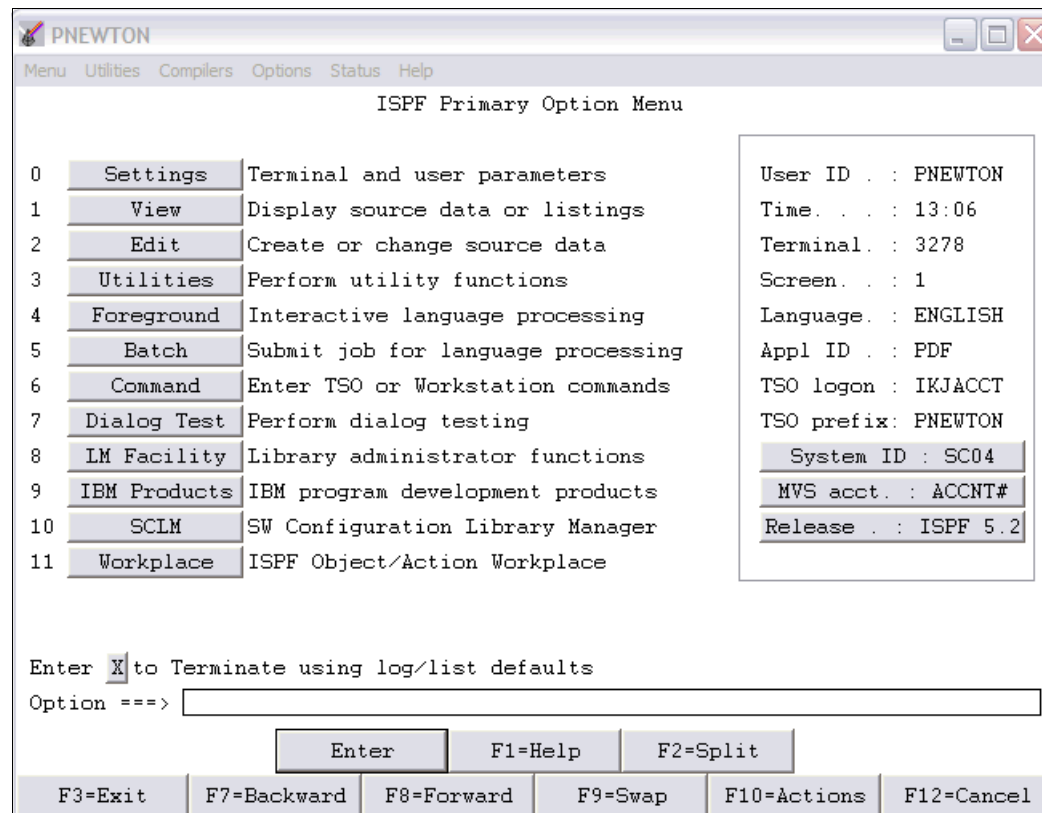
Figure 4-17 ISPF GUI
