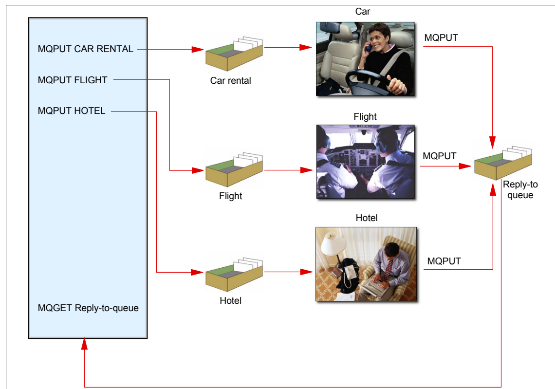
Figure 15-4 Parallel processing
