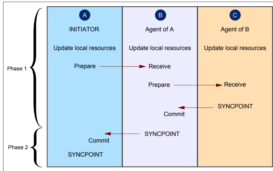
Figure 11-3 Two-phase commit
