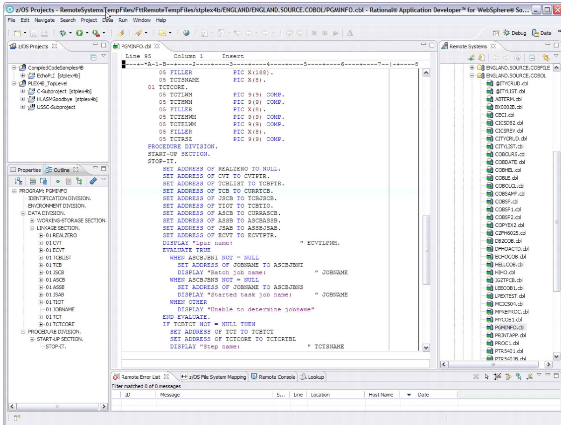
Figure 8-7 RDz page
